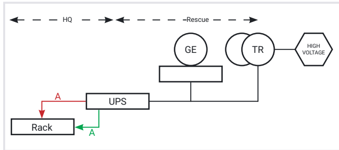
TYPE 1 - SINGLE PATH / DUAL FEED
